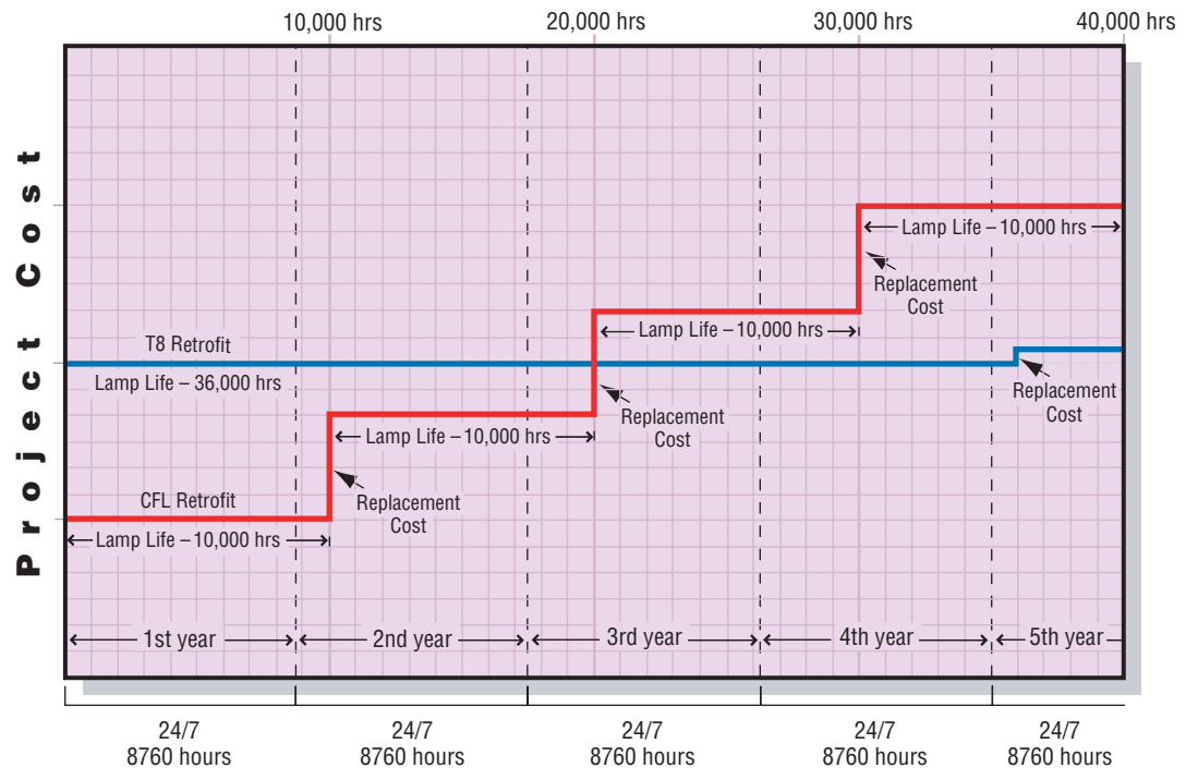
Lights Operating 24/7 (8760 hrs. per yr.)
