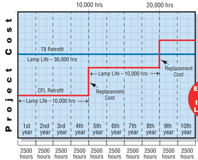
Lights Operating 1 Shift (2500 hrs. per yr.)
